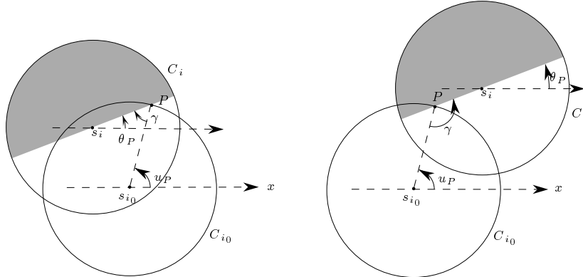
FIG. 4.4. For the proof of Proposition 4.6.
