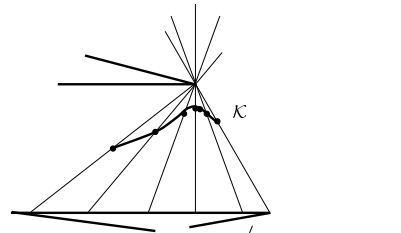
FIG. 5.6. Relevant 2-contact tracing of type (wall-endpoint) 2 , i.e., arc of ellipse.
