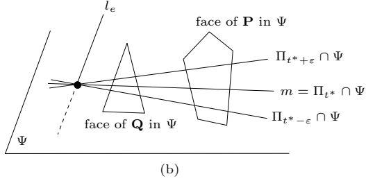
Figure 9: m is tangent to \mathbf{P} along a face in \Psi and (a) to \mathbf{Q} \cap \Psi only on l_e or (b) to \mathbf{Q} along a face in \Psi .
