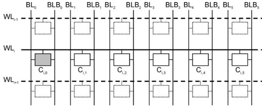
Fig. 4. A portion of an SRAM block.
