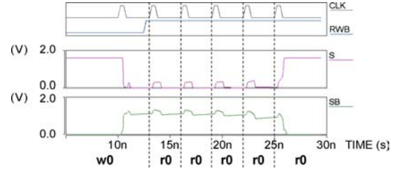
Fig. 2. A destructive read occurring after the 5th consecutive r0 operation (typical process, T = 125^\circ\text{C} , V = 1.6\text{ V} , T_{\text{cyc}} = 3\text{ ns} , R = 1.5\text{ M}\Omega ).
