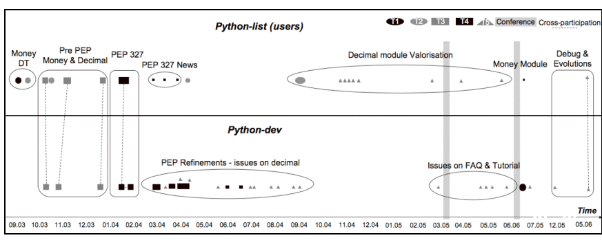
Figure 2. Temporal view of the PEP 327 design process
