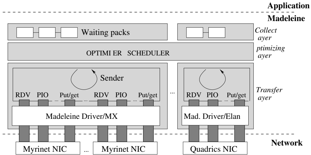
Figure 1. NEWMADELEINE architecture.
