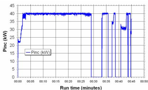
Figure 4: Couplers commissioning.
