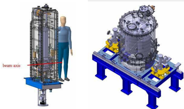
Figure 2: One of the 12 cryomodules A and 1 of the 7 cryomodules B.
