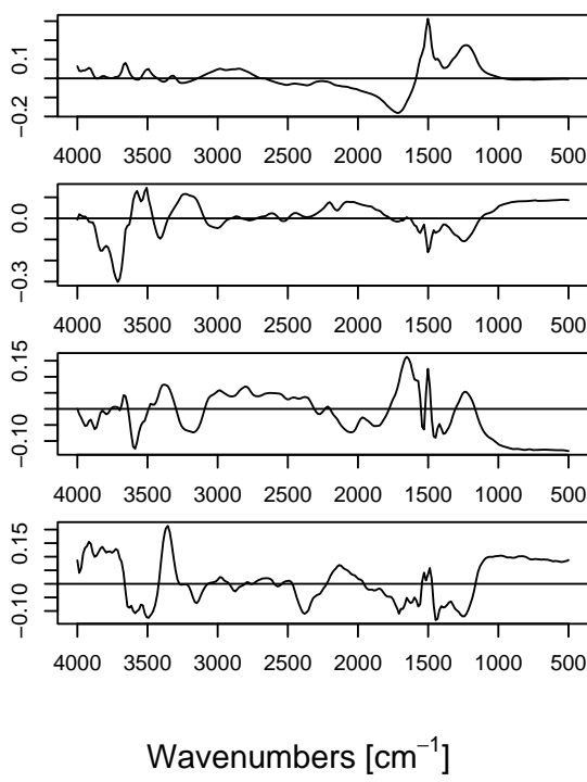
Figure 10: The four last selected loadings for PLSR in the case of Wine.
