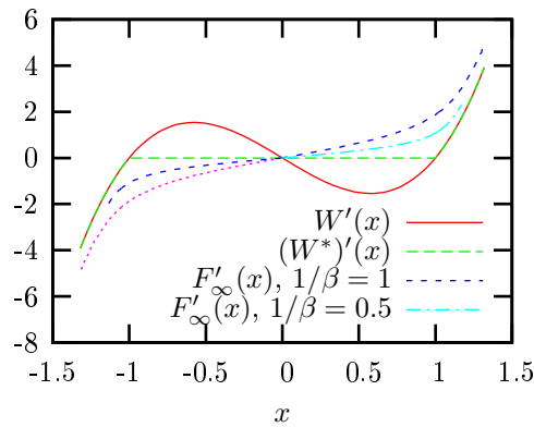
Figure 11: F'_\infty(x) for different temperatures, in the case of the double-well potential (50).
