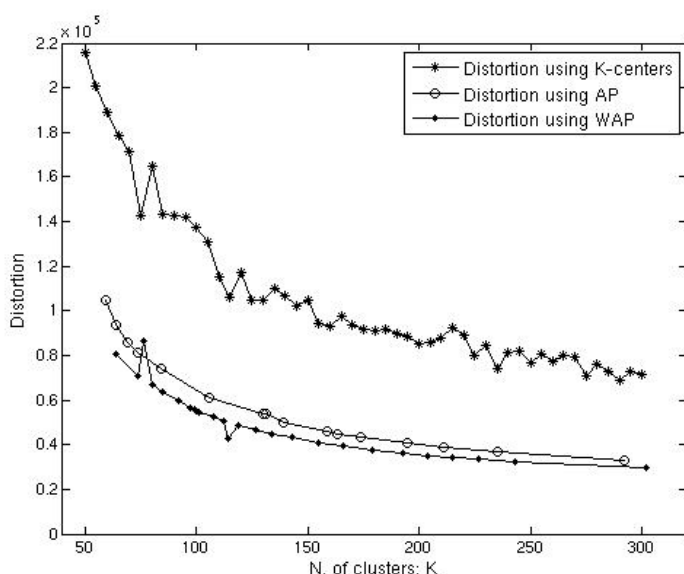
FIG. 1 – Distortion of hierarchical AP and K -centers on real-world jobs
