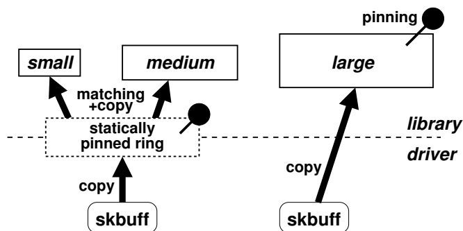
Fig. 2. Open-MX receive strategies.
