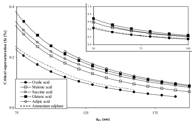
Fig. 5. Critical supersaturation as a function of dry particle diameter for the five \alpha, \omega -dicarboxylic acids studied.
