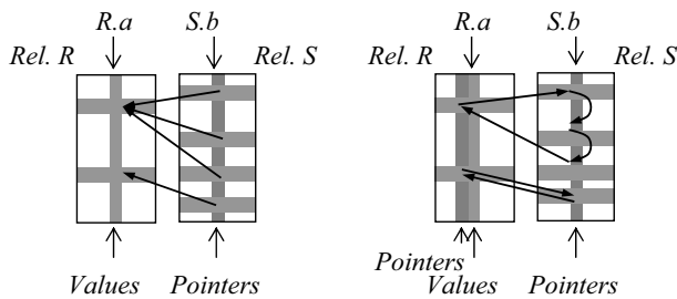
a. Domain Storage. b. Ring Storage. Figure 1: Storage models for foreign keys.
