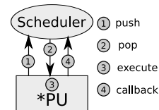
Fig. 4. Execution model
