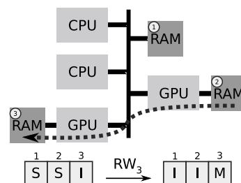
Fig. 2. Coherence protocol
