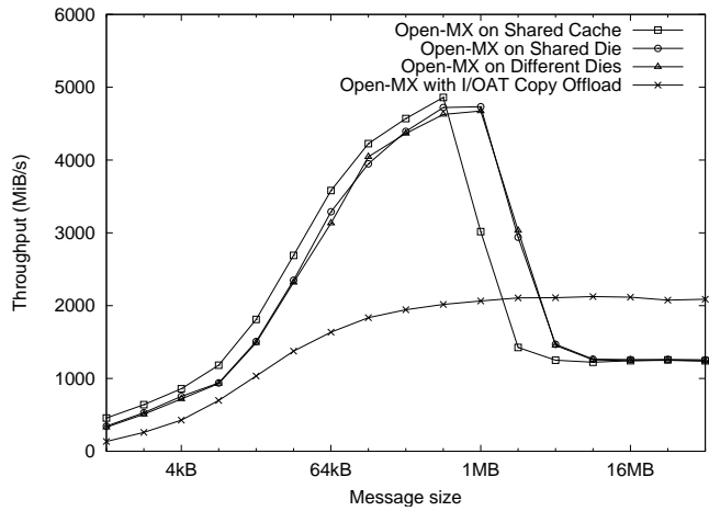
Fig. 7. IMB PingPong performance over OPEN-MX depending on process binding.
