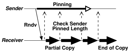
Fig. 4. Overlapped Pinning in Single-Copy communication.
