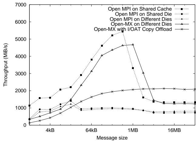
Fig. 9. Compared IMB PingPong performance over OPEN MPI and OPEN-MX depending on process binding.
