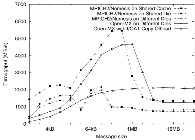
Fig. 8. Compared IMB PingPong performance over MPICH2-NEMESIS and OPEN-MX depending on process binding.
