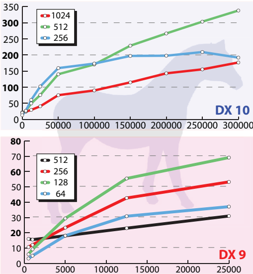
Figure 9: Speedup with respect to [5] for several LOD's of the horse model (with originally 300,000 triangles). Top: DX10 implementation (G80) Bottom: DX9 implementation (G6)
