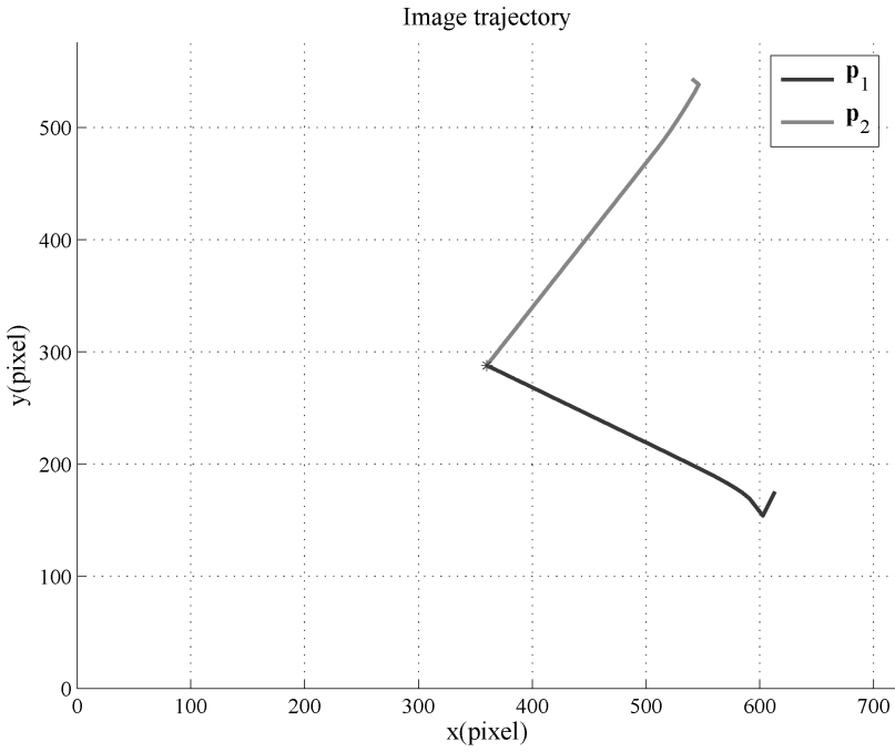
Figure 4. Image trajectories of points P_1 and P_2 during the first simulation.
