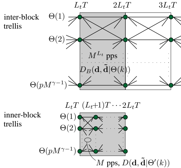
Fig. 2. Merging of inter- and inner-block trellis for simplified detection with l = 1 (pps - paths per state)
