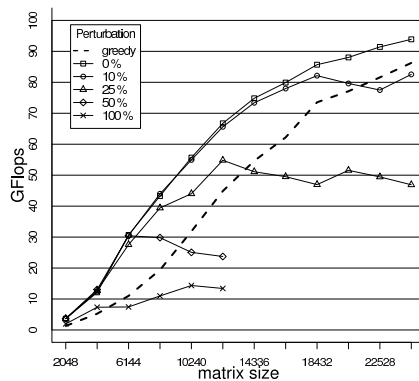
Fig. 4. Impact of the model accuracy
