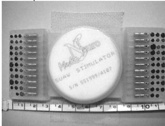
Fig. 1 The implant with its ceramic box where the electronic is encapsulated, and the connectors : 2 common anodes and 12 cathodes for epimysial stimulation, 4 anodes and 4 cathodes for neural stimulation.
