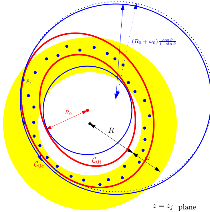
Figure 5: For the proof of Lemma 7
