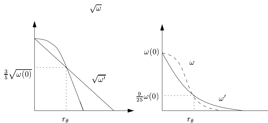
Figure 4: Relative position of \omega and \omega'
