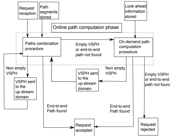
Figure 2: HID-MCP based on local improvement
