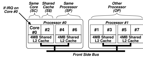
Figure 4. Processors and caches in the experimentation platform (OS-numbered).
