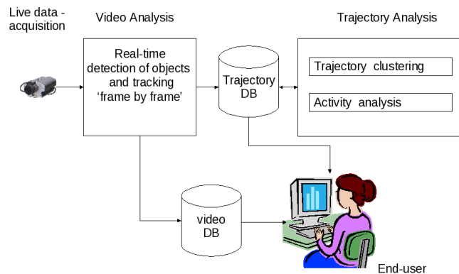
Fig. 1. General architecture.
