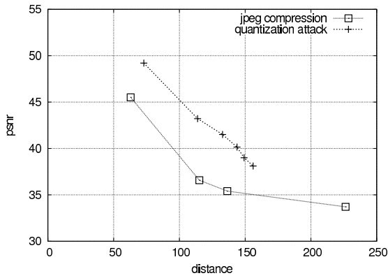
Fig. 1. Attacking SCD
