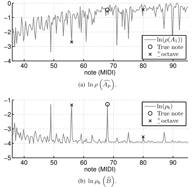
Fig. 6. \ln \rho(\widehat{A_1}) (top) and \ln \rho_b(\widehat{B}) (bottom) as a function of a single-note model (true note: Ab_4 ).
