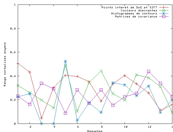
Fig. 7. Retrieval results with 15 blob queries for 53 objects of the CAVIAR project by using SIFT descriptor, edge histogram, dominant color and covariance matrix.
