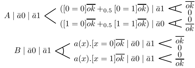
Figure 1: Execution trees for A | C and B | C
