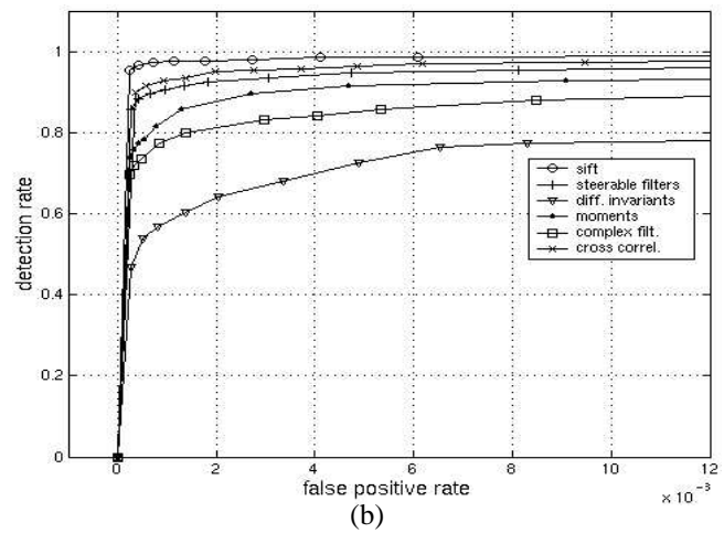
Figure 1: Evaluation for an image rotation of 45°. (a) Descriptors computed for Harris points. (b) Descriptors computed for Harris-Laplace points.
