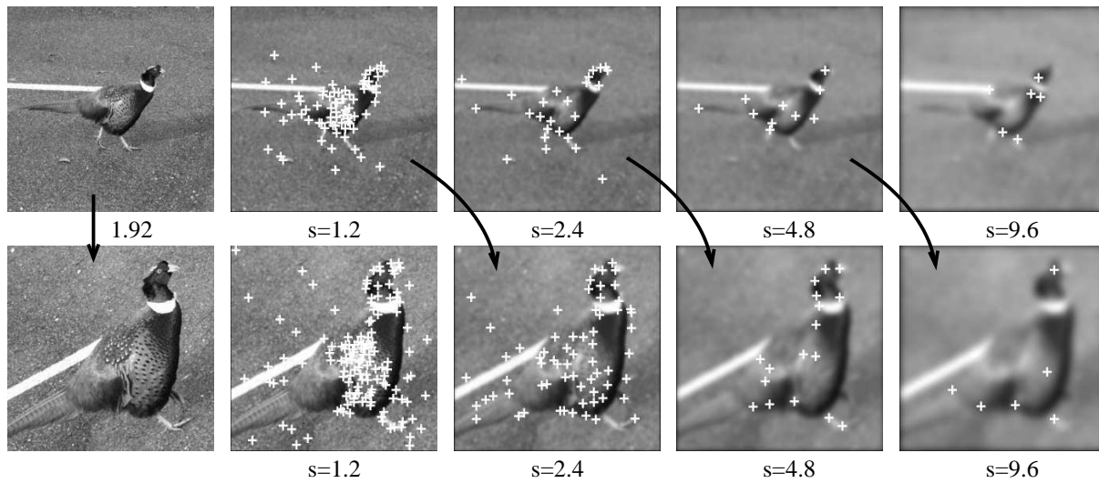
Figure 5: Points detected on different resolution levels with the Harris-Laplacian method.
