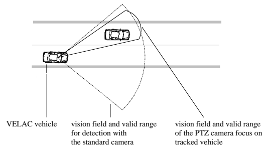
Fig. 1. PTZ camera used for tracking.
