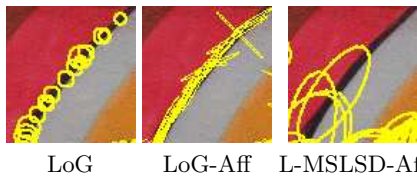
Fig. 4. Output of LoG detector on part of a graffiti image: the standard LoG detector (left), affine-invariant LoG (middle) and L-MSLSD-Aff (right).
