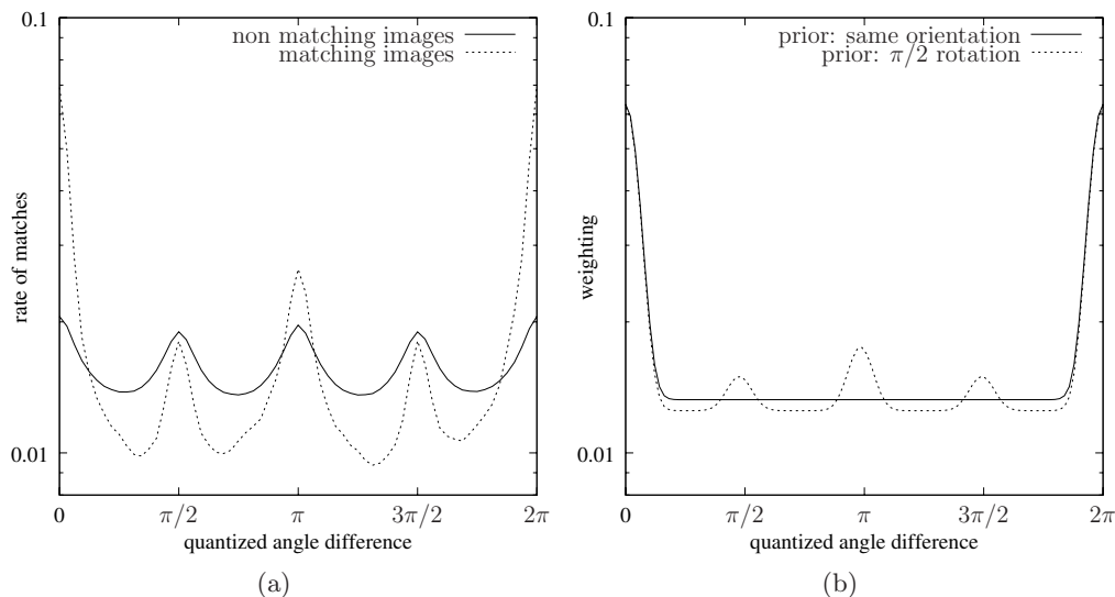
Fig. 9. (a): histogram of \delta_a values accumulated over all query images of the Holidays dataset; (b): weighting function applied in the g_j computation.
