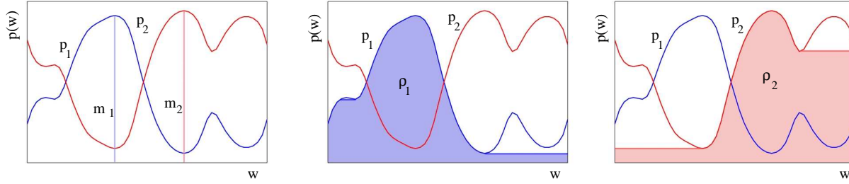
Fig. 4. Example of greyscale reconstruction. (left) Initial functions p_1 = p(z_1|w) , p_2 = p(z_2|w) , and markers m_1 and m_2 . (middle) Greyscale reconstruction \rho_1 of p_1 from m_1 . (right) Greyscale reconstruction \rho_2 of p_2 from m_2 . Since \rho_1 is by definition a unimodal function, enforcing the difference between p_1 and \rho_1 to be small reduces the secondary modes of p_1 .
