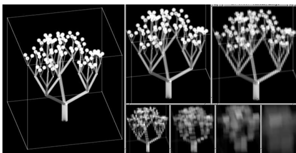
Figure 4: 256 3 volume and lower levels in the octree, down to 4 3 . On an Indigo 2 , the building costs 8 sec, and the rendering 20 sec for the first picture, 12 and 10 for the two next at resolution 444x444.
