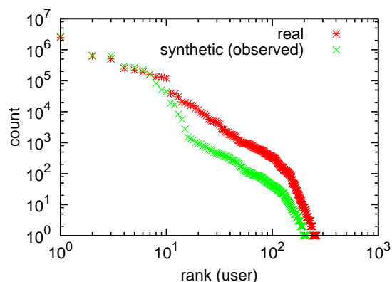
Fig. 9: Access frequency of users of synthetic trace
