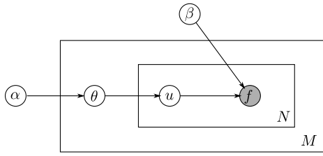
(a) LDA model assuming latent causes.
