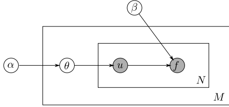
(b) LDA model assuming causes are observed.
