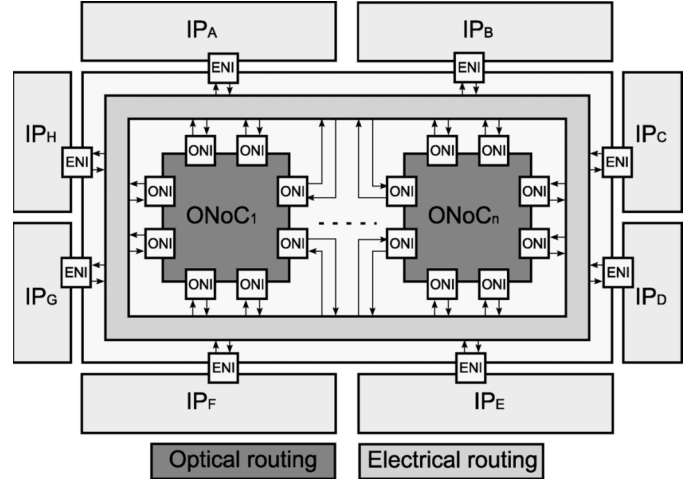
Fig. 2. Multi-ONoC architecture interconnecting eight IPs through n ONoCs.
