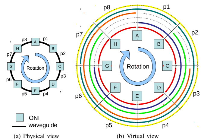
Fig. 1. Example of ORNoC highlighting multiplexed wavelengths implementing connections.
