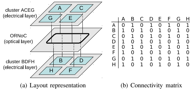
Fig. 4. 3D architecture.
