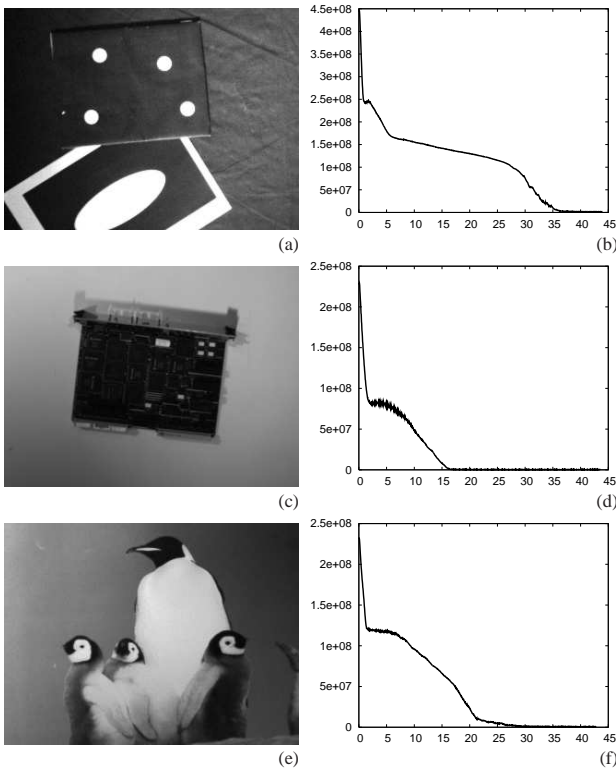
Fig. 6. Fourth experiment. Same positioning task wrt to various objects. Objects considered (left column); Cost functions (right column) ( x axis in second).
