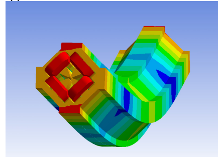
Figure 1: FE model of a type 4 MBQ including the coil [6] with a first mode at 281 Hz for free boundary conditions (measured at 264 Hz).
