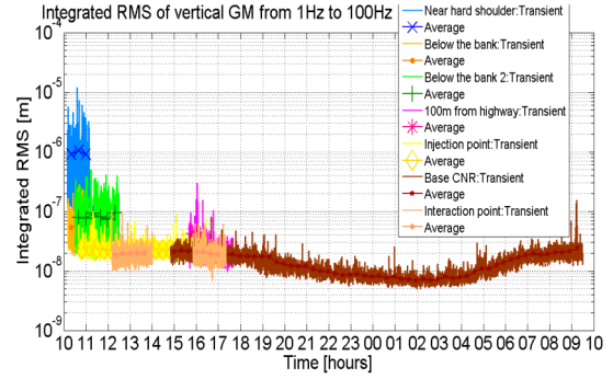
Figure 7: Vertical RMS of ground motion for all the points integrated in the frequency range [1; 100Hz].
