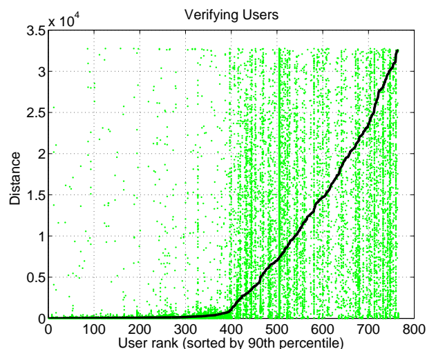
Figure 5: After two weeks, we plot the 90th percentile of the shortest distance between the IP-IDs on a ring of 2^{16} elements of the first Skype and BitTorrent packets received from a verifiable user, sorted by increasing 90th percentile (curve). There is one dot per verification experiment. We verify 400 users out of 765 users.
