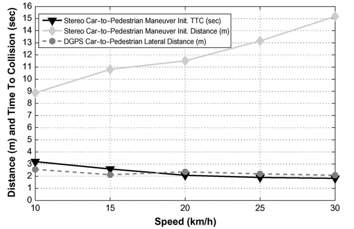
Fig. 11. Average stereo TTC (in seconds) and stereo longitudinal distance (in meters) before starting the avoidance maneuver and maximum DGPS car-to-pedestrian lateral distance.
