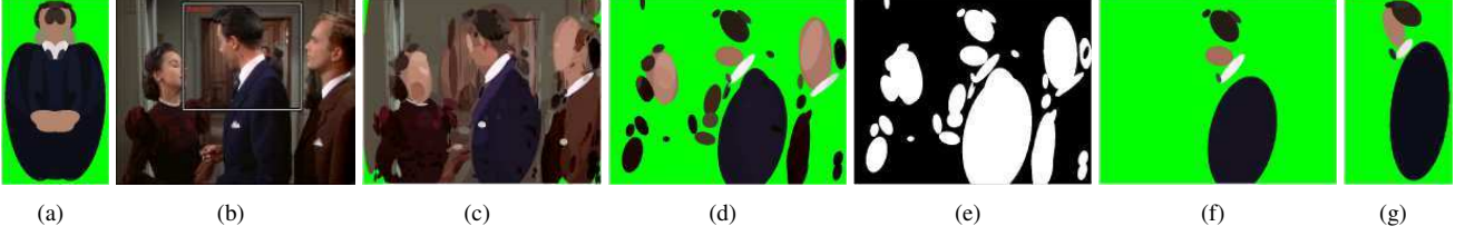
Figure 5. Illustration of the detection process. (a) Given Actor model. (b) Input frame and obtained detection for given Actor model with the proposed method. (c) MSCR features on the input frame. (d) Refined set of blobs for the given actor at given scale, based on appearance. (e) Binary map which can be used to reject some of the windows without processing, in practice we use separate binary maps for head and torso features. (f) The features in the image which were finally matched and considered for scoring for the final detection window as shown in (b). (g) The corresponding matched cluster centers in the given actor model.
