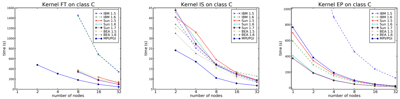
Figure 1: Execution time of the computation intensive kernels (FT, IS and EP) for various JVMs on the Gigabit Ethernet cluster
