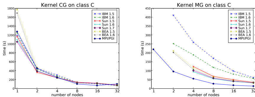
Figure 2: Execution time of the communication intensive kernels (CG and MG) for various JVMs on the Gigabit Ethernet cluster
