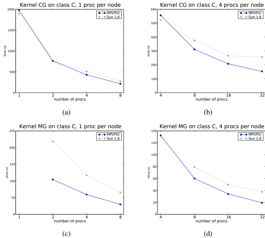
Figure 3: Execution time of the communication intensive kernels (CG and MG) on the SCI cluster
