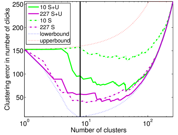
Figure 7. Evaluation of hierarchical clustering error based on different distance metrics, the true number of characters is eight.
