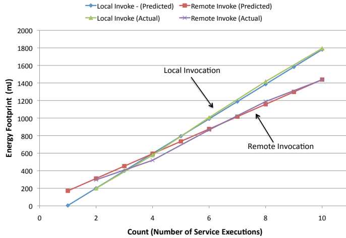
Fig. 7. The predicted and actual energy footprints of the structural health monitoring application when the radio operates at a 10% duty cycle and \text{Period} = 1000ms .
