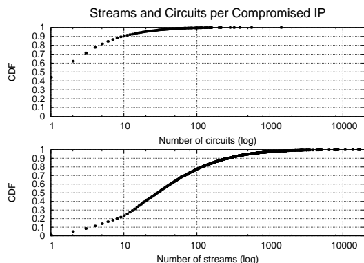
Figure 3: Distribution of de-anonymized circuits (top) and streams (bottom) per de-anonymized IP. Once we de-anonymize an IP, we are able to de-anonymize multiple circuits and streams using the domino effect.
