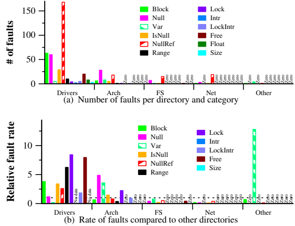
Figure 4: Faults in Linux 2.4.1
