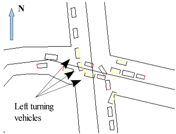
Figure 9: "complex" deadlock
